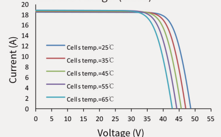
Current-Voltage (710W)
